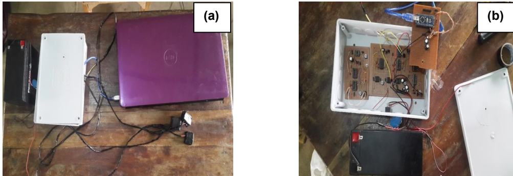
Fig. 4. (a) Complete set-up of an eddy current test device (b) The Micro-controller
