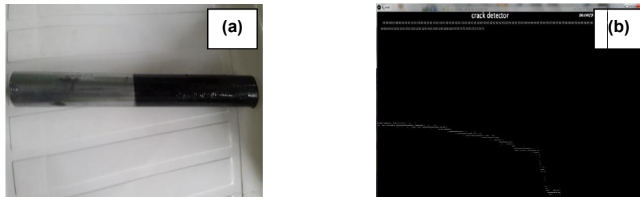
Fig. 8(a). Showing a half-coated pipe tested for coating flaws (b) Result of test galvanized pipe with coating flaws
