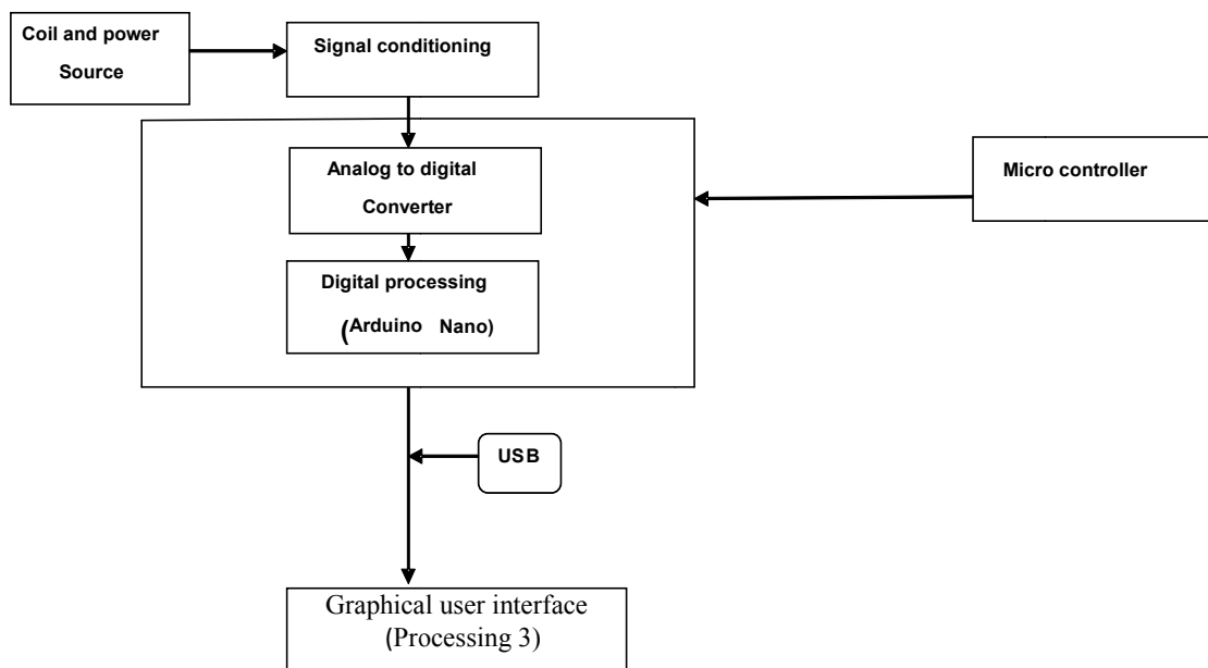
Fig. 2. Flow diagram denotes principal for eddy current testing device
