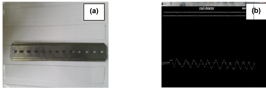
Fig.1 (a). The metal plate used to calibrate the device (b) Result showing the twelve holes on tested device
