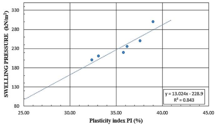
Fig. 3. Swelling pressure vs plasticity index
