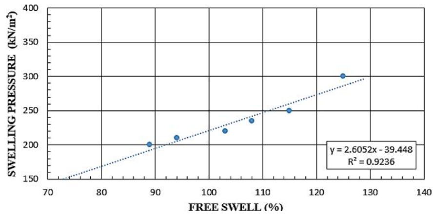
Fig. 2. Swelling pressure vs free swell
