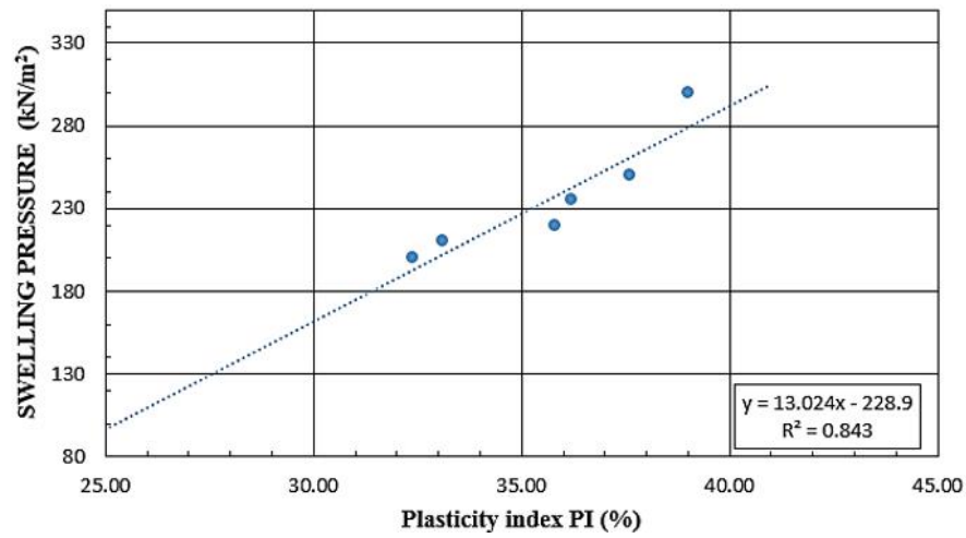
Fig. 3. Swelling pressure vs plasticity index
