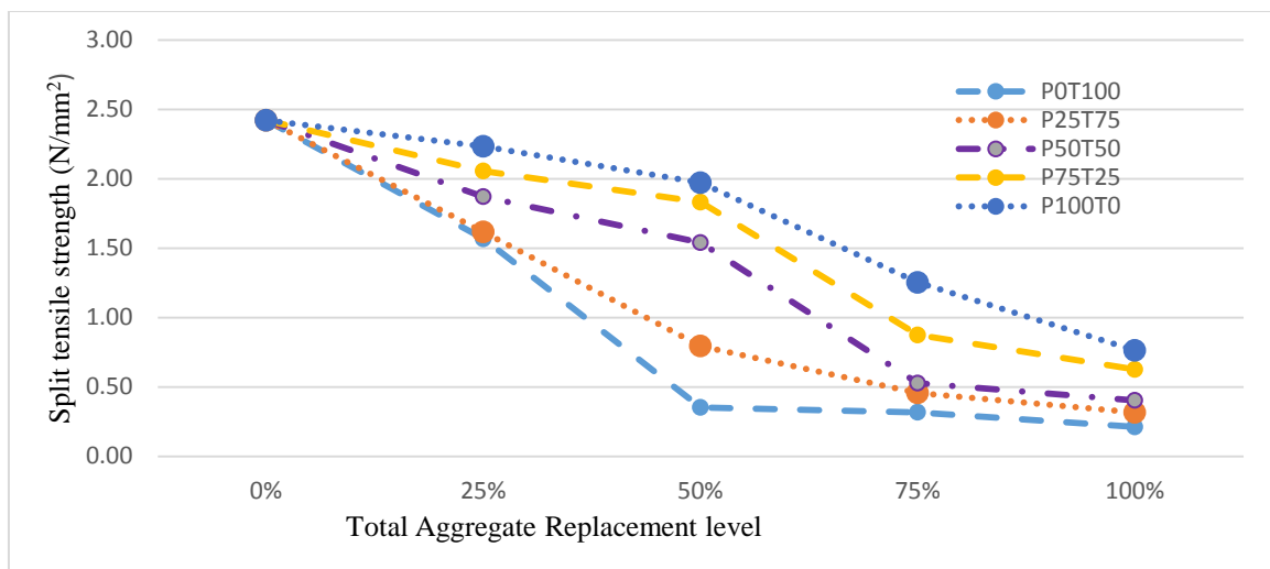
Fig. 6. Effect of PKS-Tire content on split tensile strength
