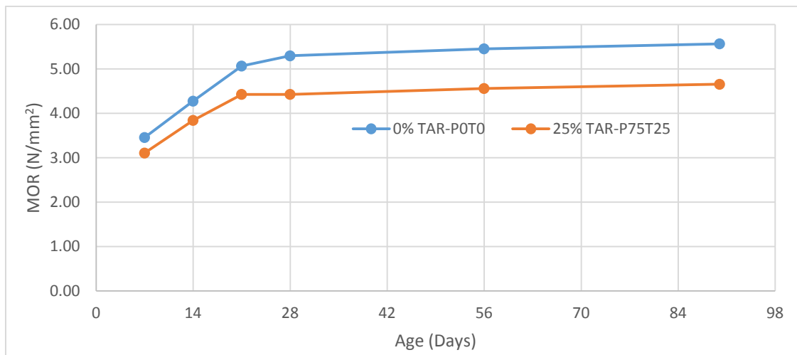
Fig. 5. Modulus of Rupture with age of curing
