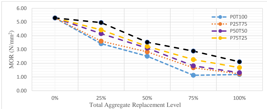
Fig. 4. Variation of MOR with increase in PKS-tire content
