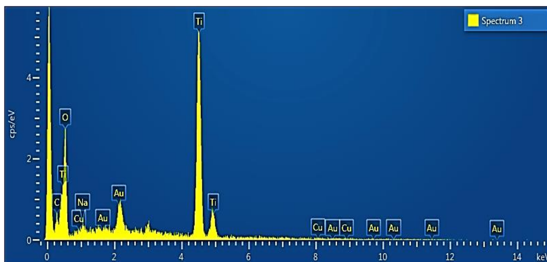
Fig. 2. EDX spectra of \text{TiO}_2 nanoparticles
