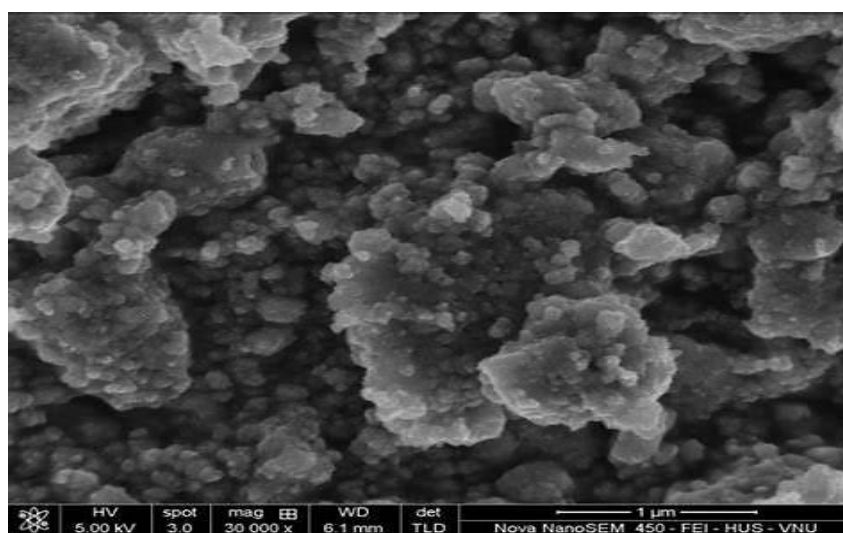
Fig. 1. SEM images of Ni-doped \text{TiO}_2 Nanoparticles at 1 \mu\text{m}
