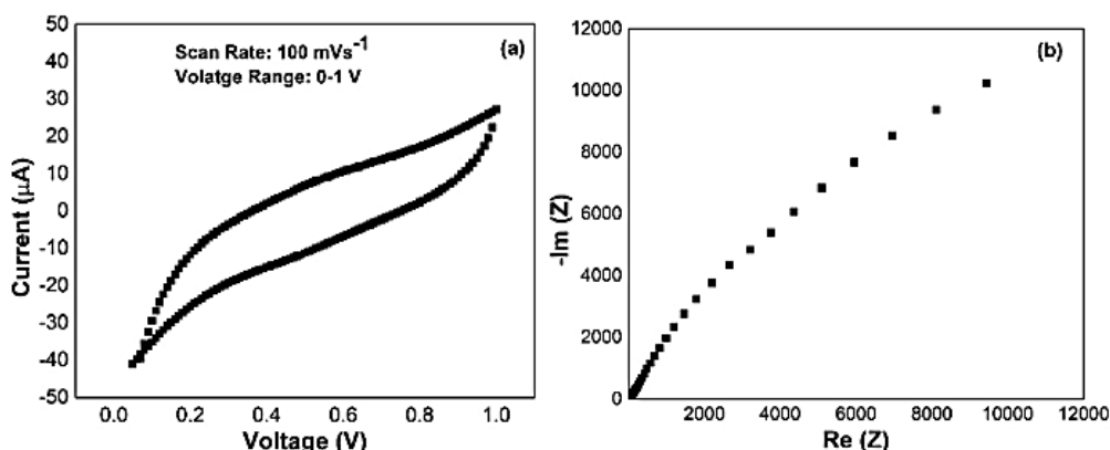
Fig. 4. (a). CV curve of TiO 2 electrodes in voltage range of 0–1 V at scan rate of 100 mVs -1 and (b) Nyquist plot
