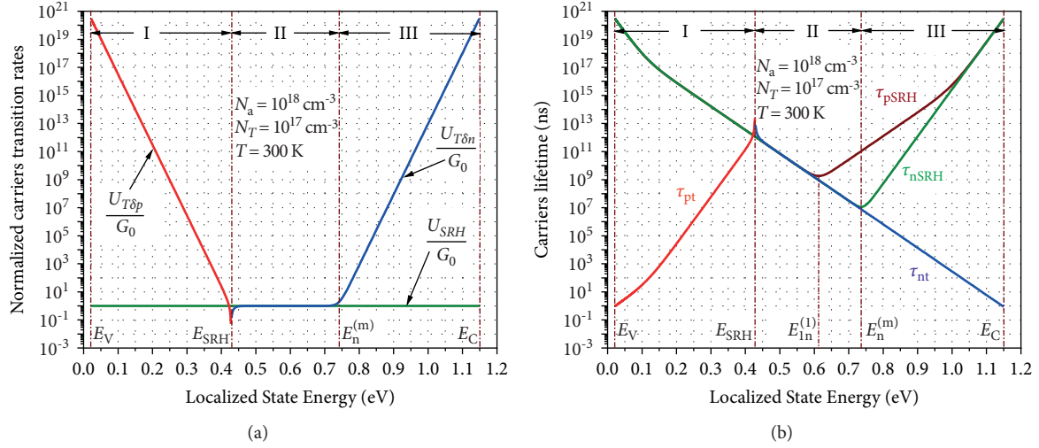
FIGURE 4: Room-temperature localized state energy dependence of (a) U_{T\delta n}/G_0 (blue curve), U_{T\delta p}/G_0 (red curve), and U_{\text{SRH}}/G_0 (green curve) and (b) \tau_{\text{nt}} (blue curve), \tau_{\text{pt}} (red curve), \tau_{\text{nSRH}} (green curve), and \tau_{\text{pSRH}} (wine curve) for the system discussed in Figure 2.
